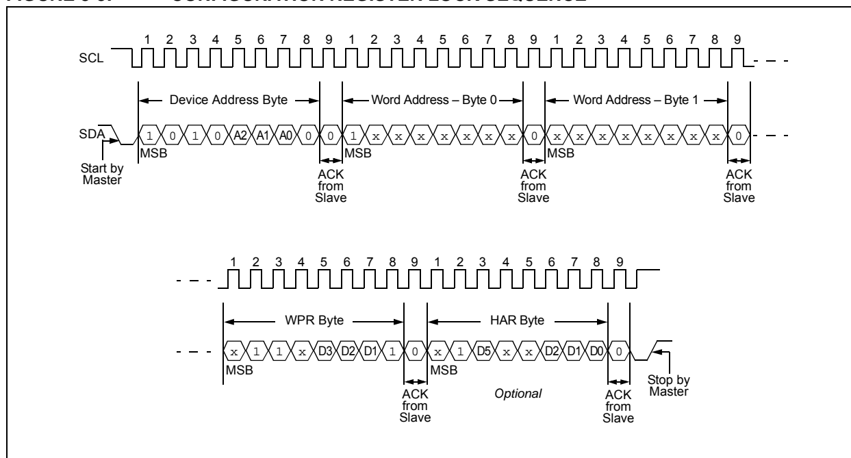
FIGURE 8-3: CONFIGURATION REGISTER LOCK SEQUENCE
