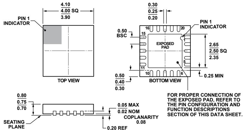
Figure 44. 20-Lead Frame Chip Scale Package [LFCSP_WQ] 4 mm × 4 mm Body, Very Very Thin Quad (CP-20-10) Dimensions shown in millimeters
