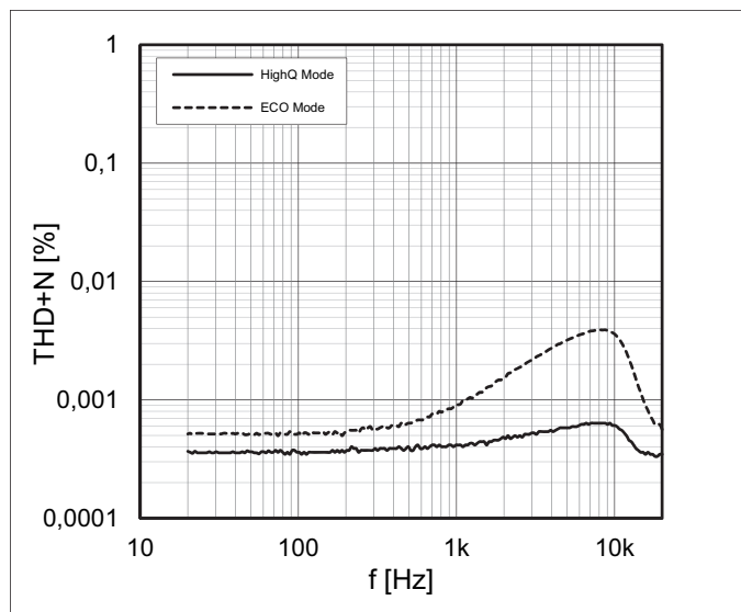
Figure 18: Line Input THD+N vs. Frequency V_{BAT} = 1.8V
