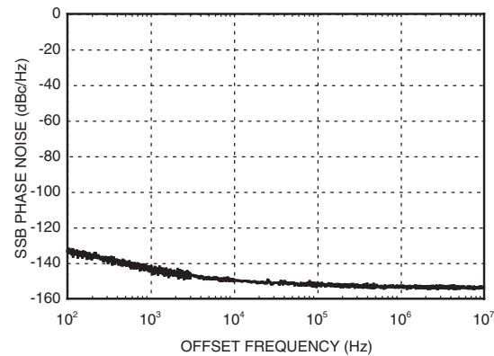
Performance, \text{Pin} = 0\text{ dBm} , T = 25^\circ\text{C}
