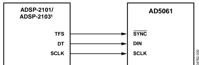
Figure 40. AD5061-to-ADSP-2101/ADSP-2103 Interface
