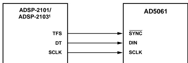
Figure 40. AD5061-to-ADSP-2101/ADSP-2103 Interface
