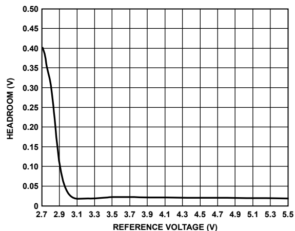
Figure 27. V_{\text{DD}} Headroom vs. Reference Voltage.
