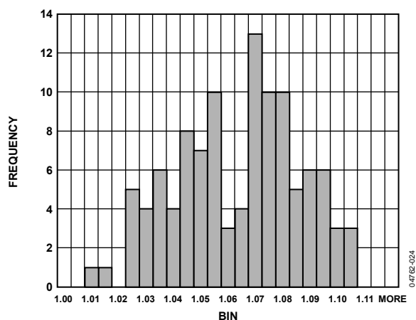
Figure 24. I_{\text{DD}} Histogram @ V_{\text{DD}} = 5\text{V}
