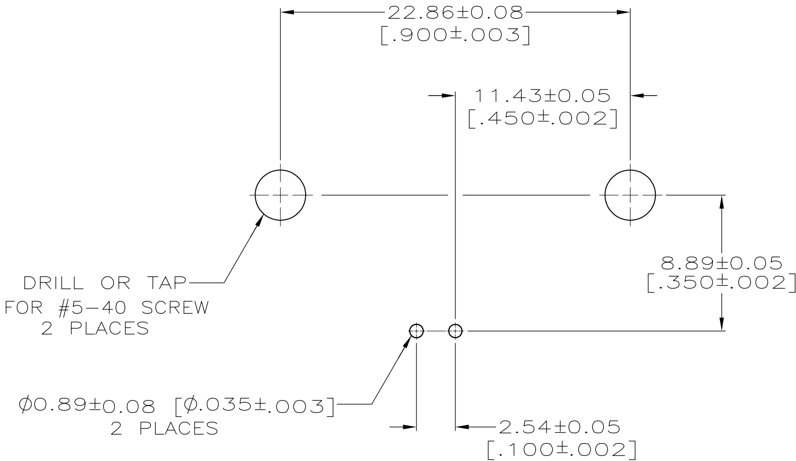
PCB CONFIGURATION
