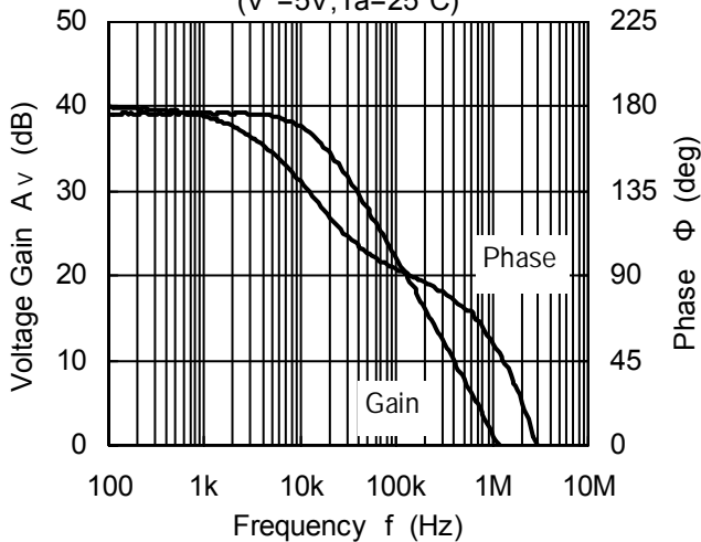
Ach Voltage Gain · Phase vs. Frequency
