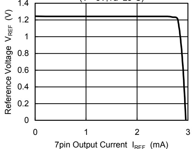
Reference Voltage vs. 7pin Output Current
