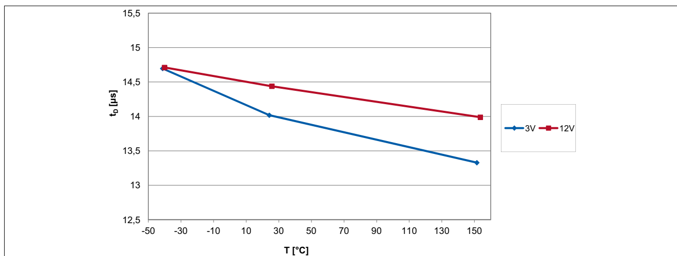
Figure 6-2 Signal Delay Time of the TLE4961-1M over Temperature
