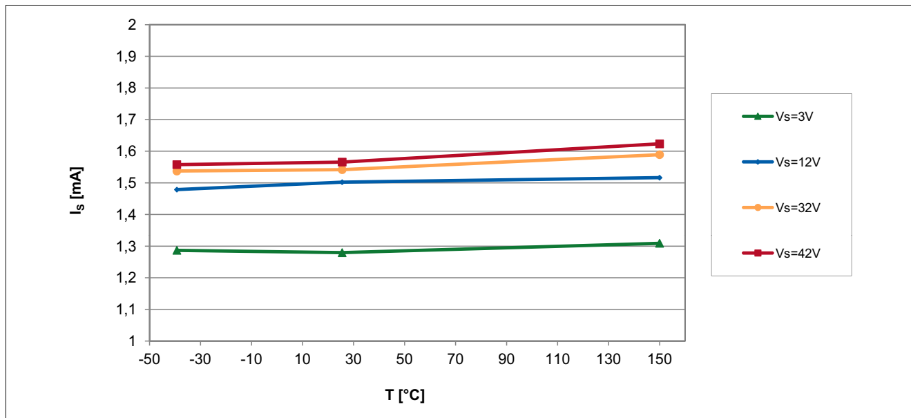
Figure 6-3 Supply Current of the TLE4961-1M over Temperature
