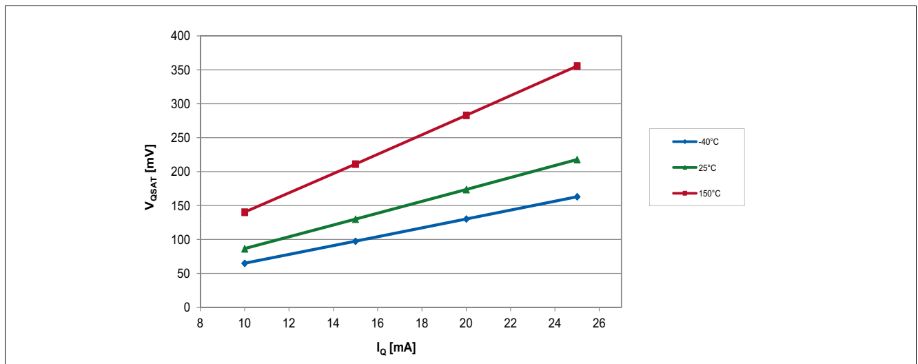
Figure 6-13 Saturation Voltage of the TLE4961-1M over Output Current
