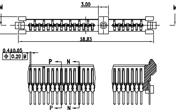
SECTION M-M
