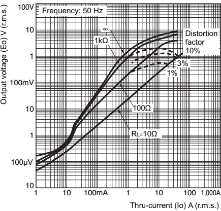
Thru-current (Io) vs. Output Voltage (Eo) (Reference Values)
