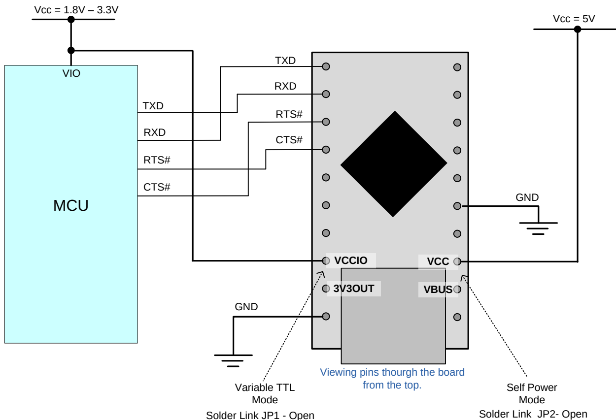
Figure 5.2 – Self-Powered Configuration
