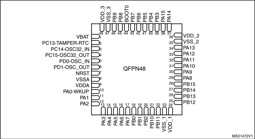
Figure 5. STM32F101xx Low-density access line UFQFPN48 pinout
