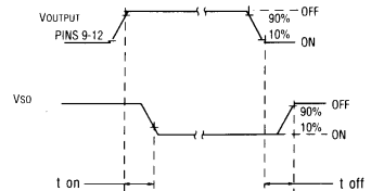
STATUS TURN-ON AND TURN-OFF TIMING (A) FIGURE 6
