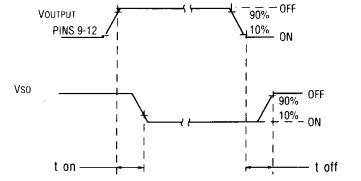
STATUS TURN-ON AND TURN-OFF TIMING (A) FIGURE 6
