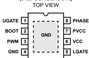
ISL6612BCB, ISL6613BCB, ISL6612BECB, ISL6613BECB (8 LD SOIC, EPSOIC)
