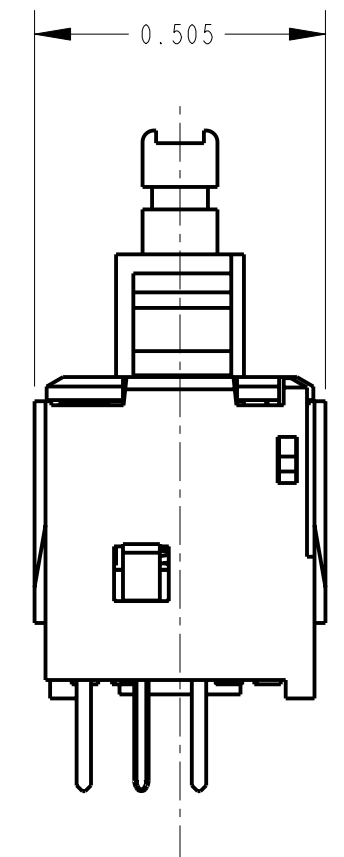
CUSTOMER DRAWING
