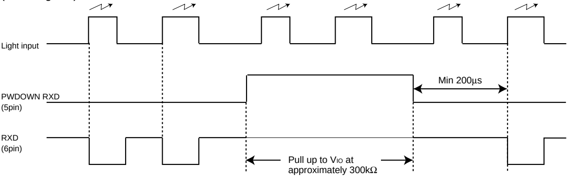
(Receiving side)
