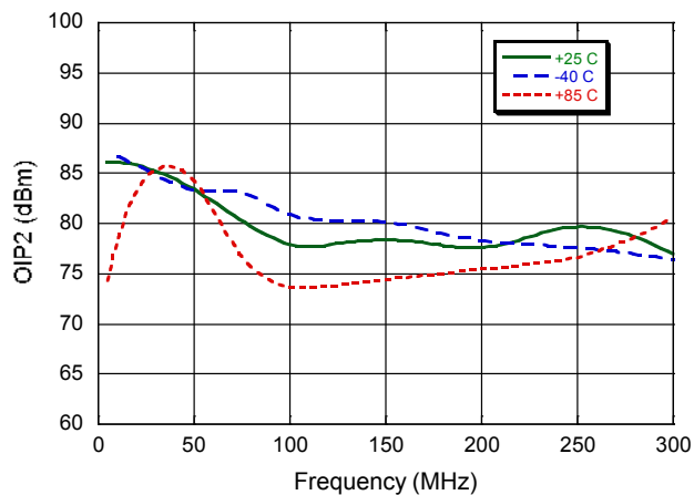
OIP2 @ P_{OUT} = 12\text{ dBm}
