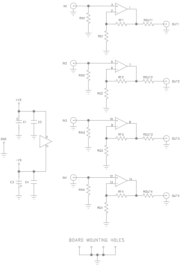
Figure 18. CEB018 & CEB017 Schematic
