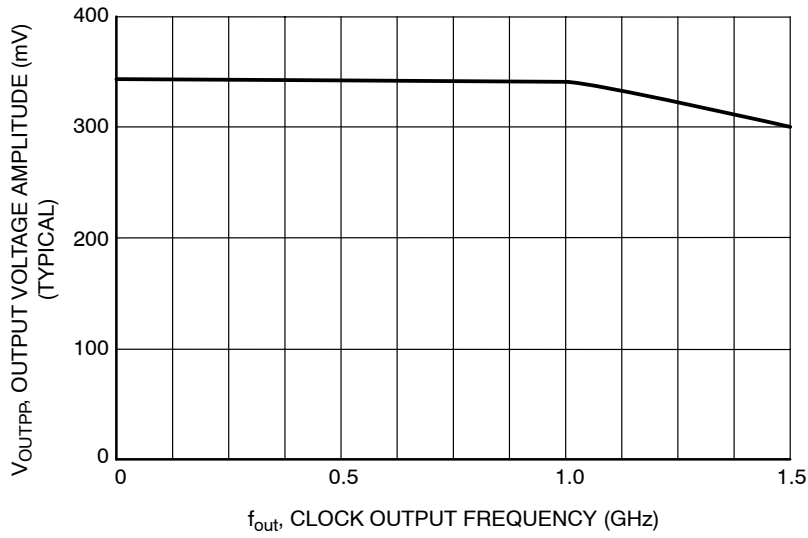
Figure 18. Output Voltage Amplitude ( V_{OUTPP} ) versus Output Clock Frequency at 25°C (Typical) f_{out} (QA/QB) = f_{in} \div n ; For n = 2, 4, 8, 16 ; f_{in} \leq 3.0 GHz For n = 1 ; f_{in} \leq 1.5 GHz
