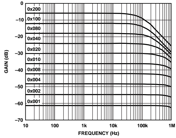
Figure 28. 100 kΩ Gain vs. Frequency vs. Code
