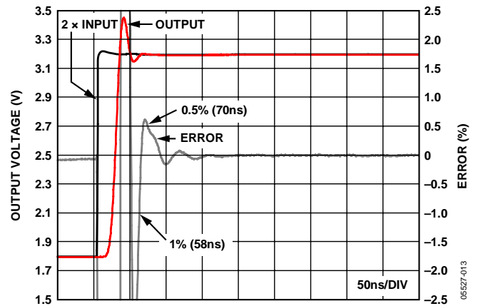
Figure 13. Settling Time
