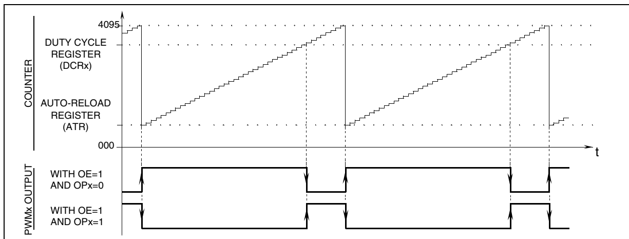
Figure 38. PWM Function
