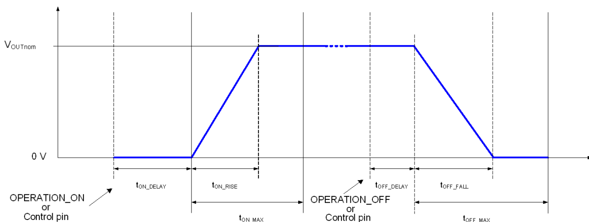
Figure 5: Power Sequencing
