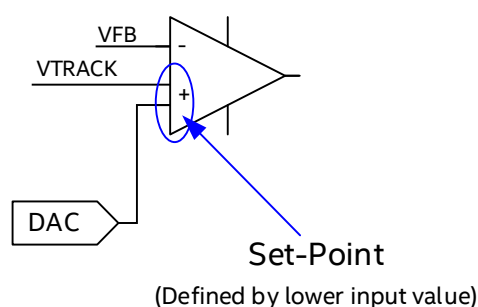
Figure 9: VTRACK Circuitry
