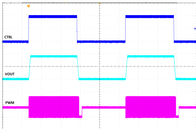
Start-up/Shutdown, CTRL At No Load, 20 ms/div
