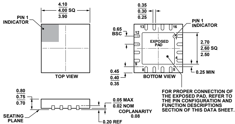
Figure 53. 16-Lead Lead Frame Chip Scale Package [LFCSP_WQ] 4 mm × 4 mm Body, Very Very Thin Quad
