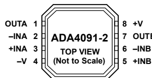
Figure 1. 8-Lead, Narrow-Body SOIC (R-8)
