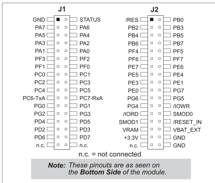
Figure 6. RCM3200 Pinouts
