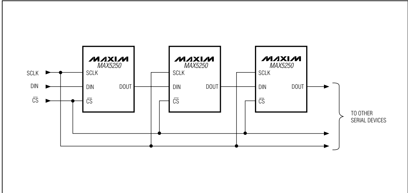
Figure 7. Daisy-Chaining MAX5250s
