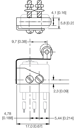
Figure 12. JM-5 Dimensions
