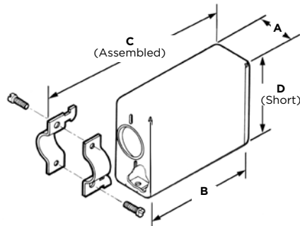
90° Cable Exit
