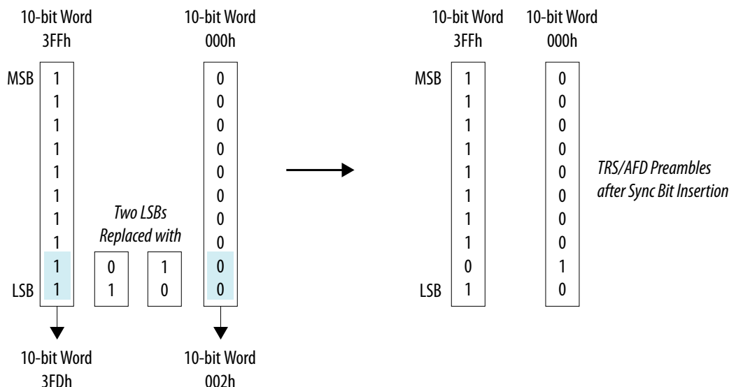
Figure 23. Sync Bits
