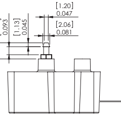
C- Barb Fitting Port B Only Configuration
