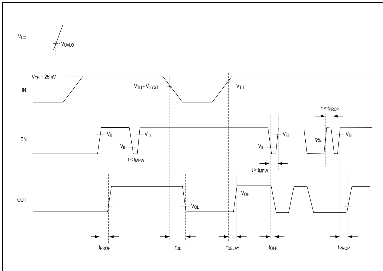
Figure 1. MAX16052/MAX16053 Timing Diagram ( C_{CDelay} = 0 )
