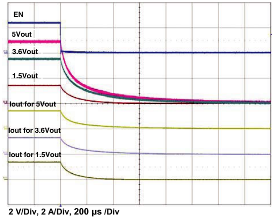
Figure 30 - Typical Fall Time C_{OUT} = 100 \mu F, C_{IN} = 4.7 \mu F, I_{OUT} = 1.5 A
