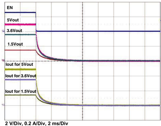
Figure 31 - Typical Turn-on Delay, Fall Time C_{OUT} = 100 \mu F, C_{IN} = 4.7 \mu F, R_{OUT} = 10 \Omega
