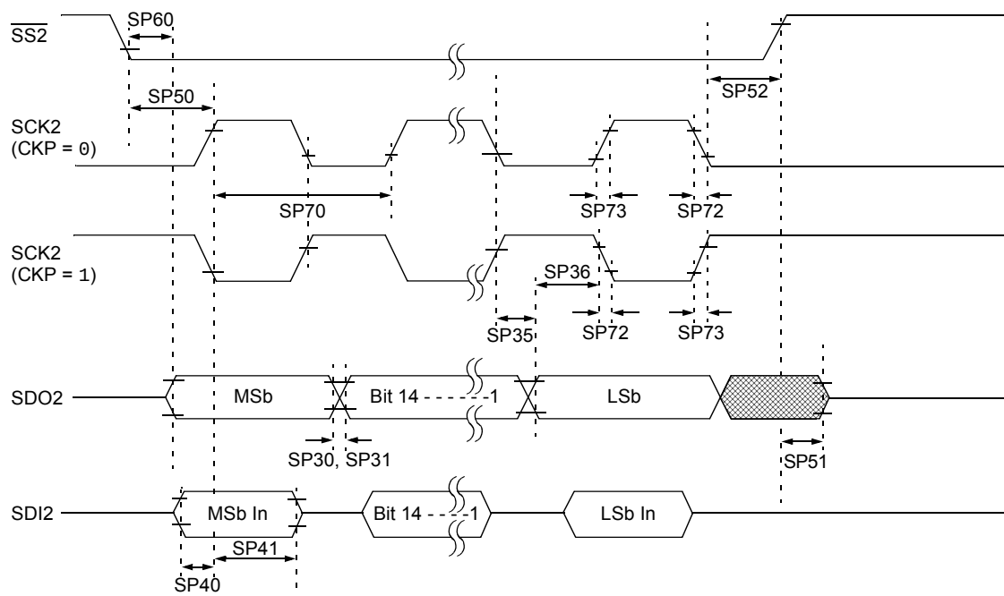
FIGURE 30-16: SPI2 SLAVE MODE (FULL-DUPLEX, CKE = 1, CKP = 0, SMP = 0) TIMING CHARACTERISTICS
