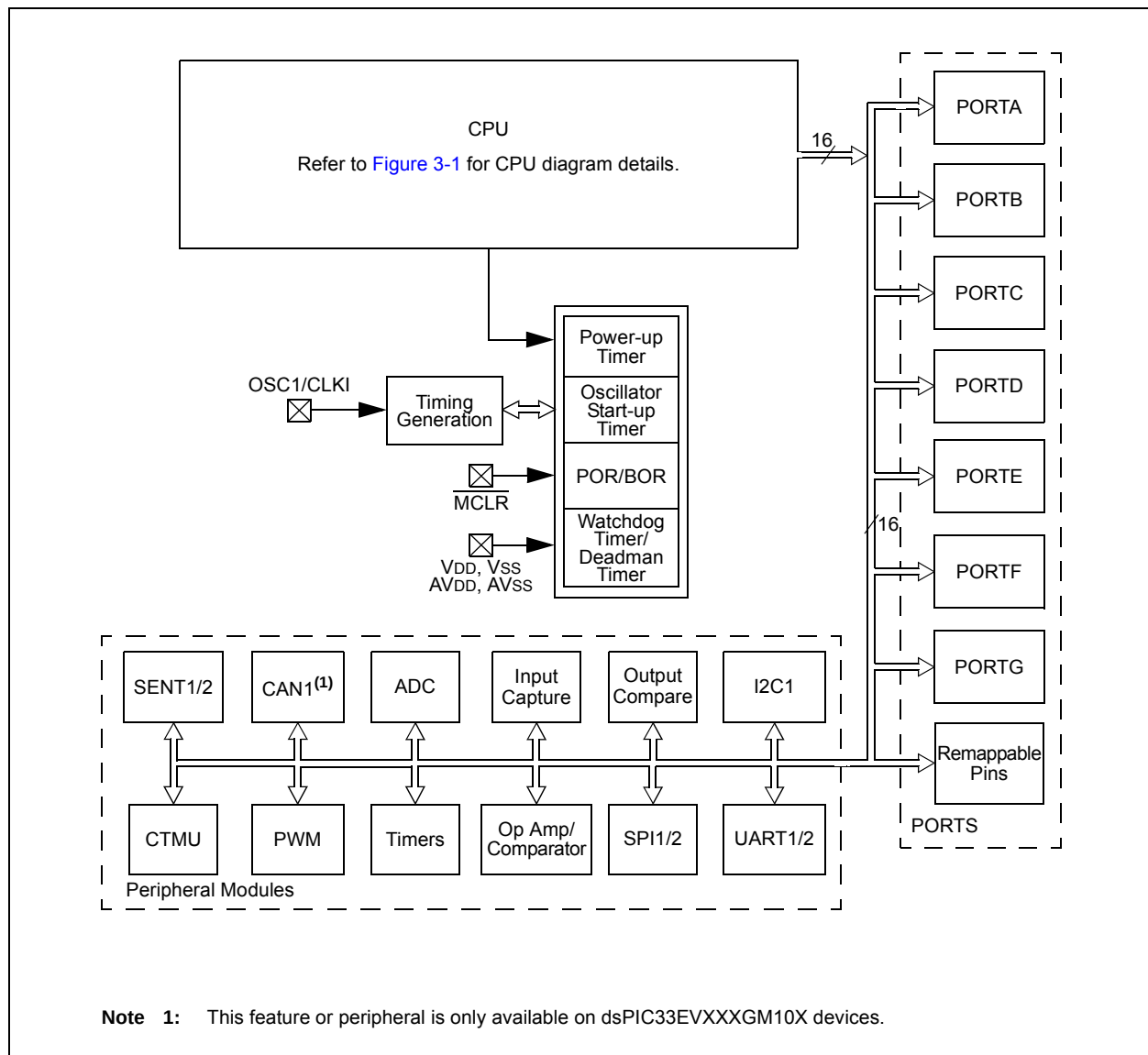
FIGURE 1-1: dsPIC33EVXXGXM00X/10X FAMILY BLOCK DIAGRAM
