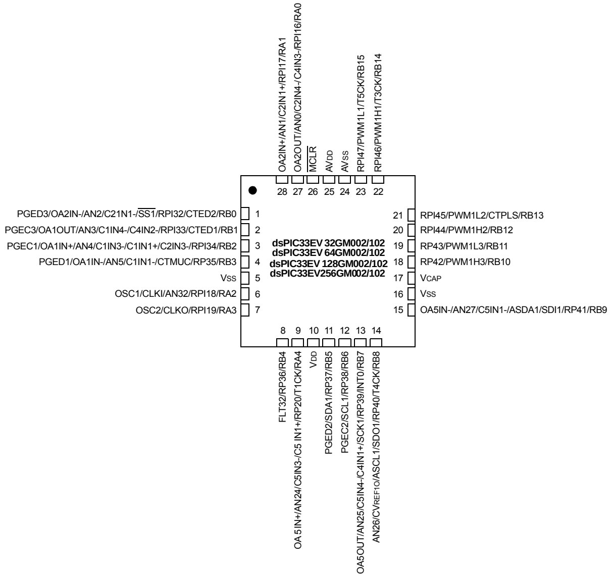
28-Pin QFN-S (1,2,3,4)
