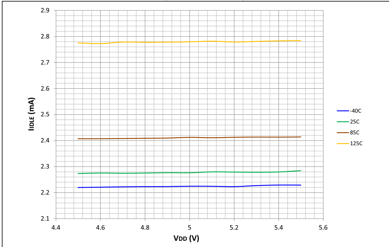
FIGURE 32-9: TYPICAL I_{IDLE} vs. V_{DD} (EC MODE, 20 MIPS)
