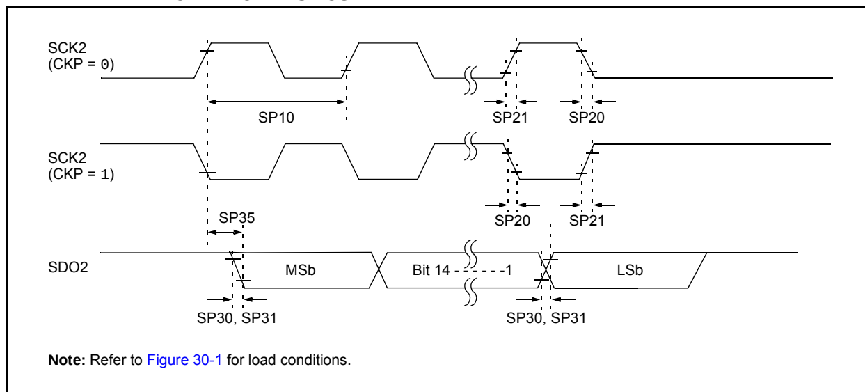
FIGURE 30-12: SPI2 MASTER MODE (HALF-DUPLEX, TRANSMIT ONLY, CKP = 0) TIMING CHARACTERISTICS
