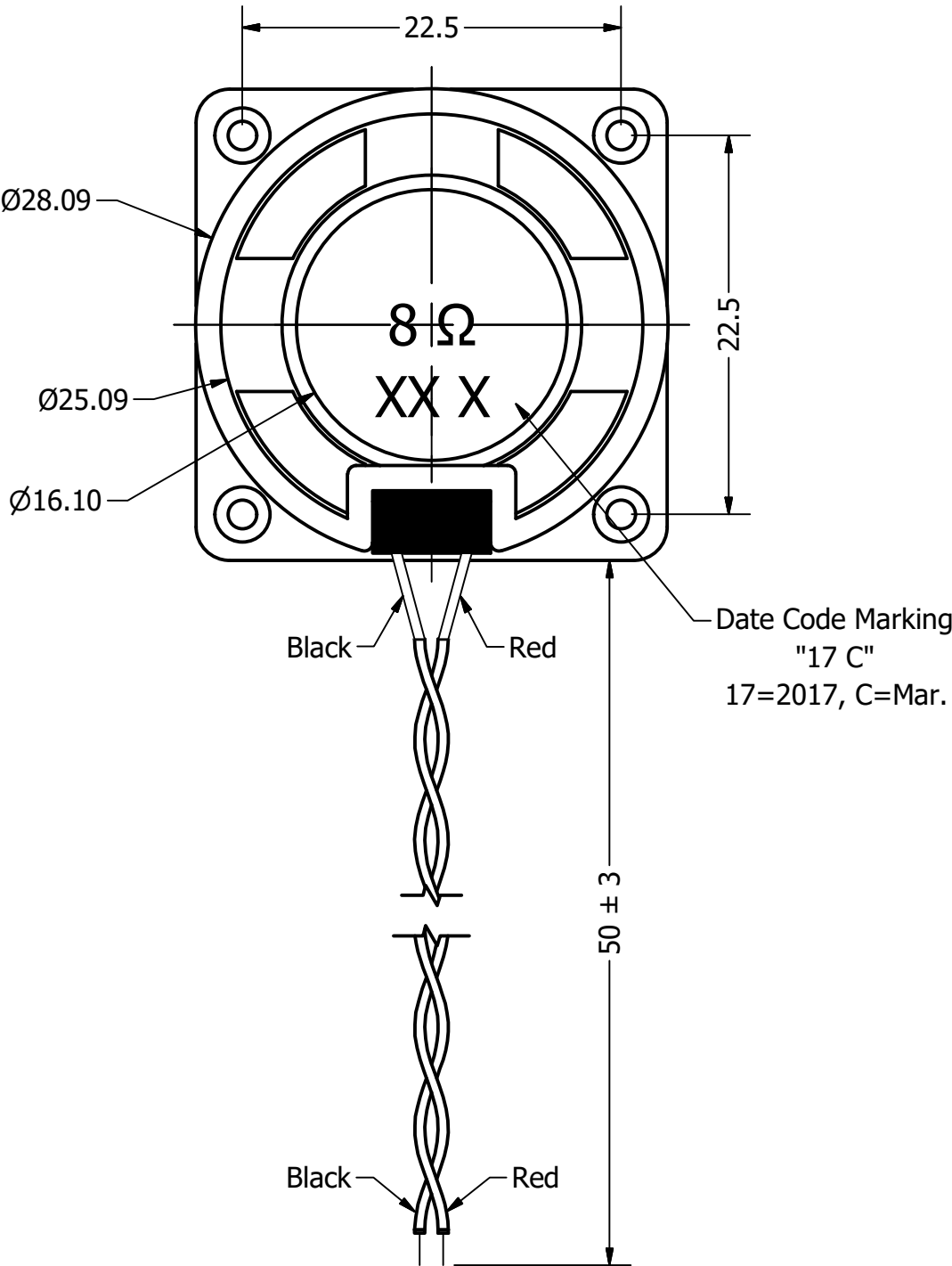
Bottom View
