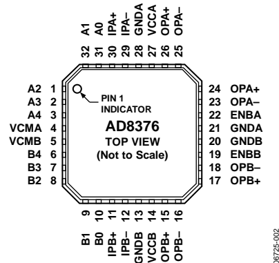
Figure 3. 32-Lead LFCSP
