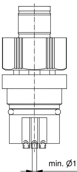
Inner view ( 2 : 1 )
