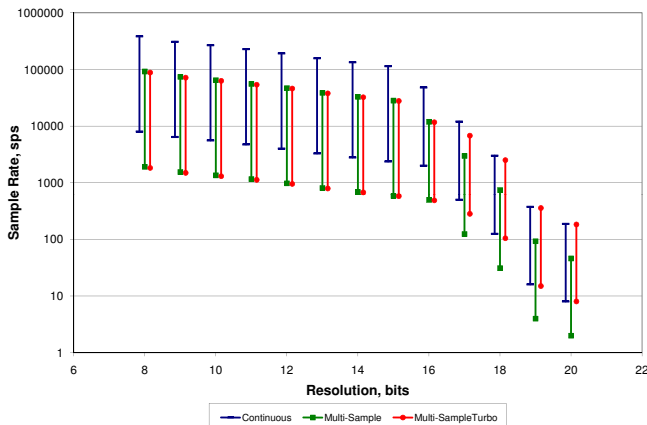
Figure 8-3. Delta-sigma ADC Sample Rates, Range = ±1.024 V
