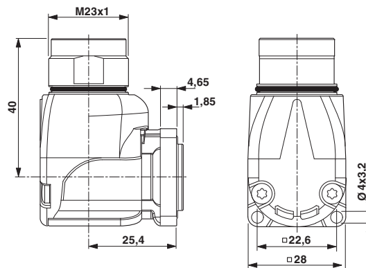
Dimensioned drawing
