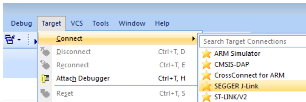
Figure 13: Debug Settings
