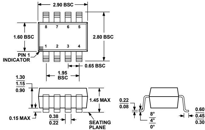
Figure 48. 8-Lead Small Outline Transistor Package [SOT-23] (RJ-8) Dimensions shown in millimeters
