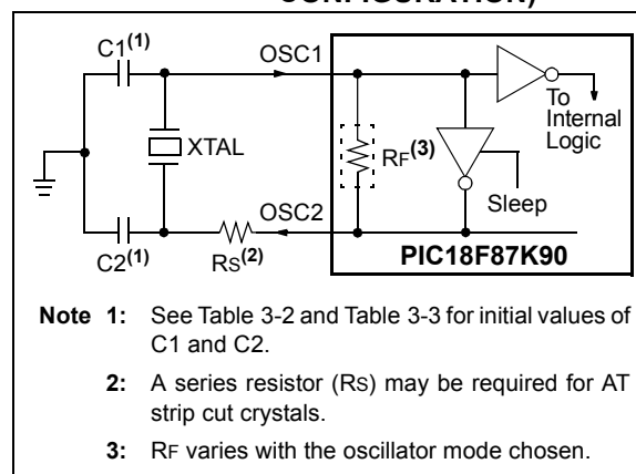
FIGURE 3-2: CRYSTAL/CERAMIC RESONATOR OPERATION (HS OR HSPLL CONFIGURATION)
