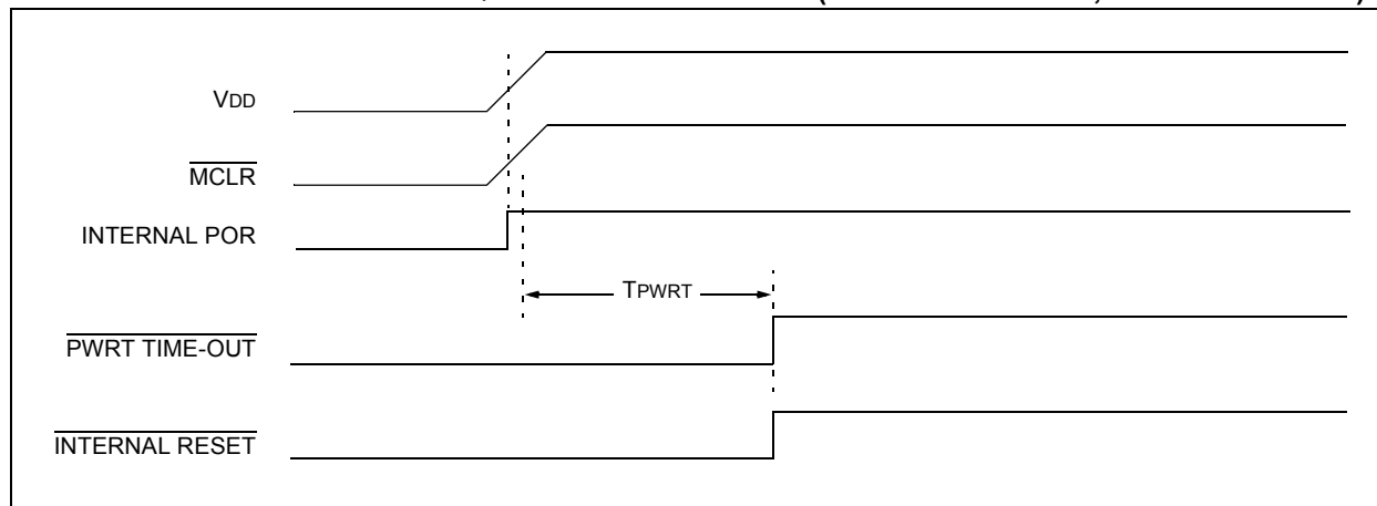
FIGURE 5-3: TIME-OUT SEQUENCE ON POWER-UP ( \overline{\text{MCLR}} TIED TO \text{V}_{\text{DD}} , \text{V}_{\text{DD}} RISE < \text{T}_{\text{PWRT}} )
