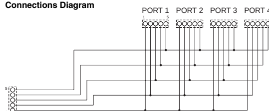
Connections Diagram
