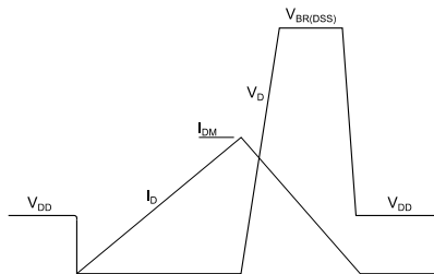
Figure 21: Unclamped inductive waveform
