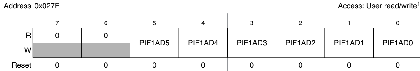
Figure 2-44. Port AD Interrupt Flag Register (PIF1AD)
