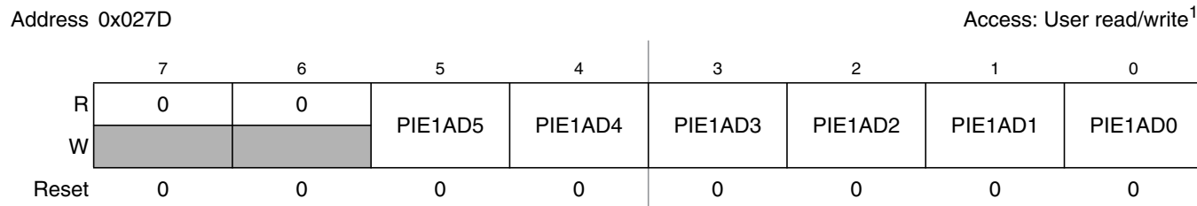
Figure 2-43. Port AD Interrupt Enable Register (PIE1AD)
