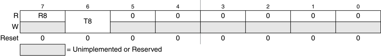
Figure 10-12. SCI Data Registers (SCIDRH)
