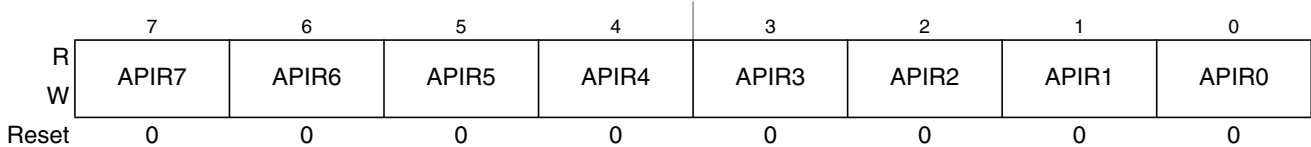
Figure 4-23. Autonomous Periodical Interrupt Rate Low Register (CPMUAPIRL)
