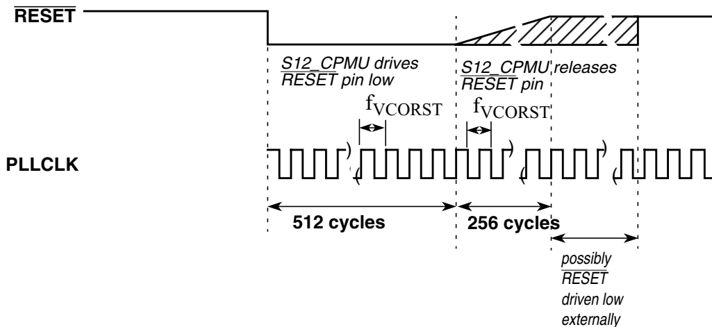
Figure 4-37. RESET Timing
